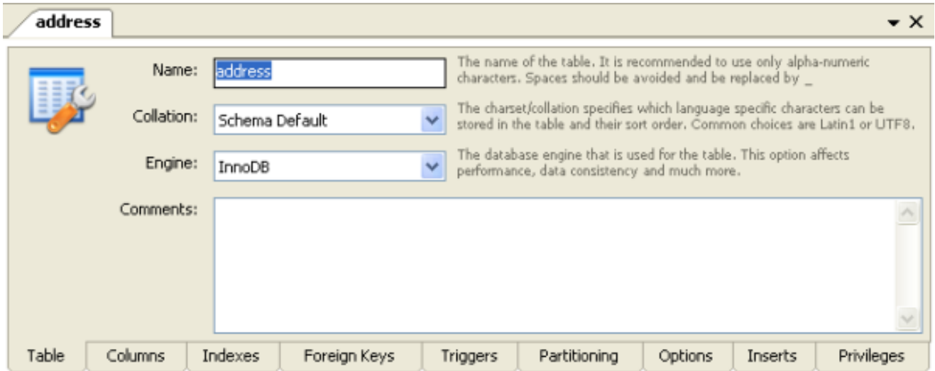
Figure 7.2. The table editor
