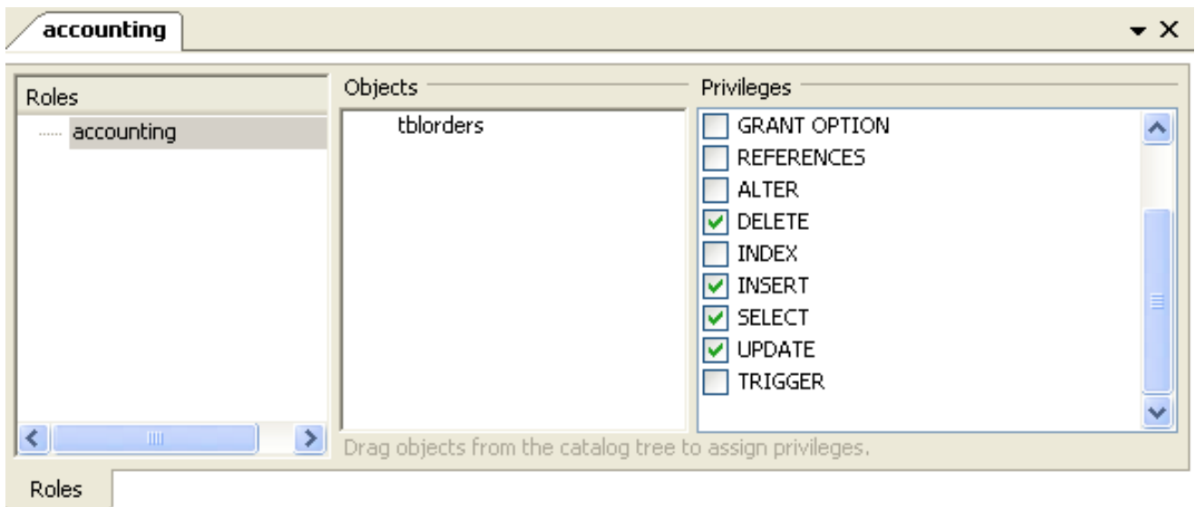
Figure 6.9. Role editor
